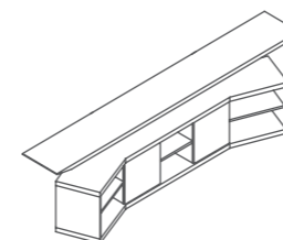
背柜 ET92 Filing Cabinet W3250*D700*H890(mm)
